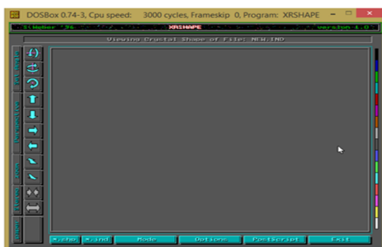
Figure 1. XRSHAPE application
